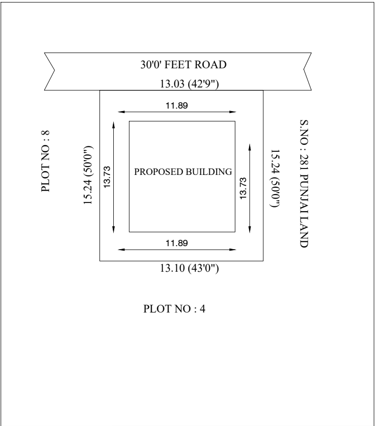
SITE PLAN
