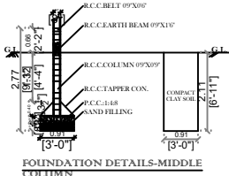
FOUNDATION DETAILS-MIDDLE COLUMN
