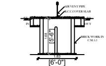
SEPTIC TANK DEATILS-SECTION
