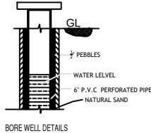
BORE WELL DETAILS
