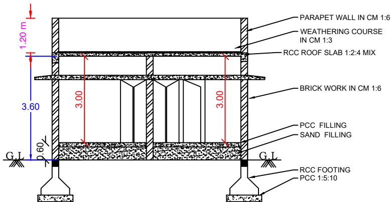
SECTION AB
