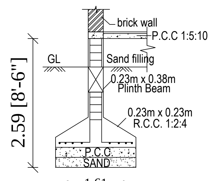
FOUNDATION DETAILS
