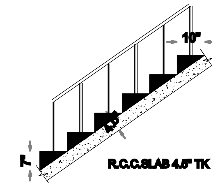
STAIRCASE DETAILS
