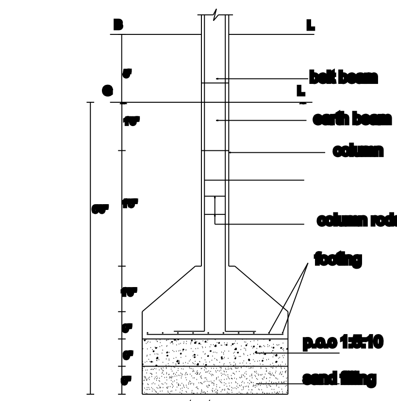
FOUNDATION DETAILS
