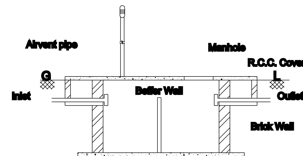
SEPTIC TANK PLAN DETAILS
