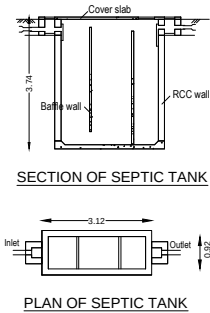
PLAN OF SEPTIC TANK
