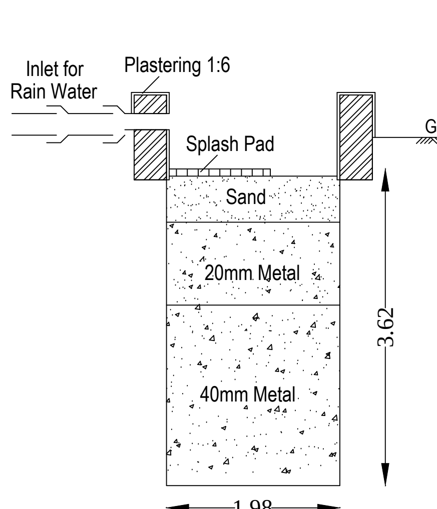
RAIN WATER PERCOLATION PIT
