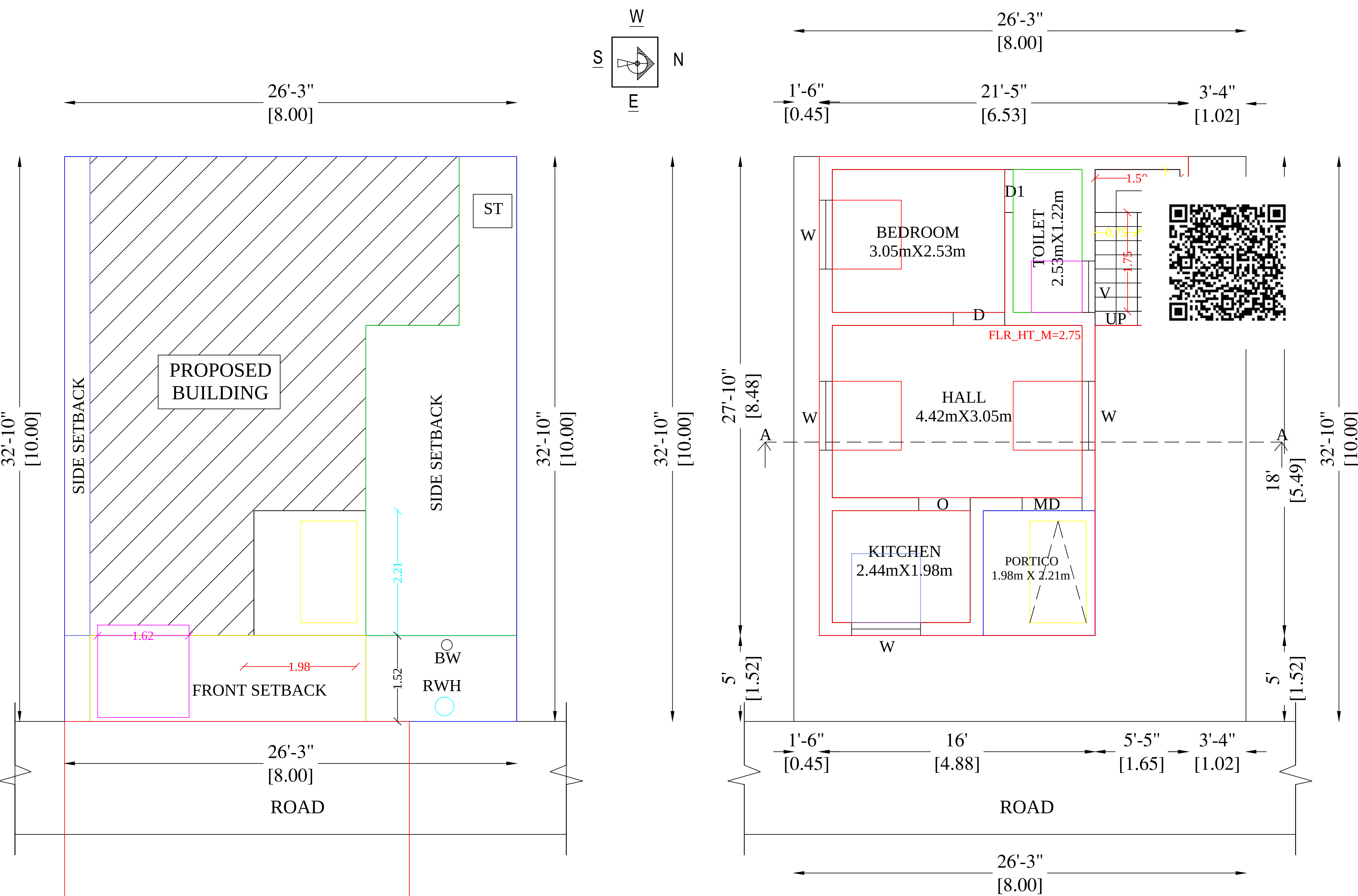
SITE PLAN
