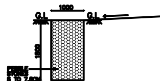
SECTION OF PEBBLE TRENCH SCALE : 1: = 100
