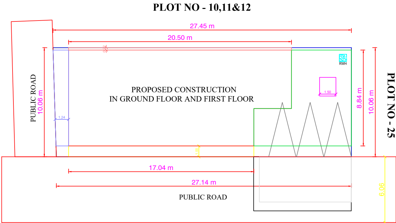
SITE PLAN
