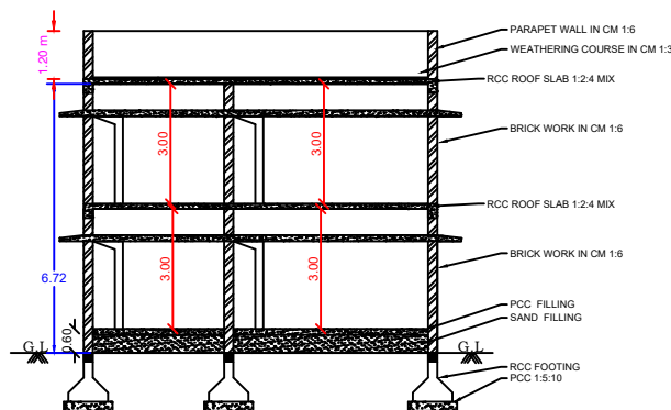
SECTION AB
