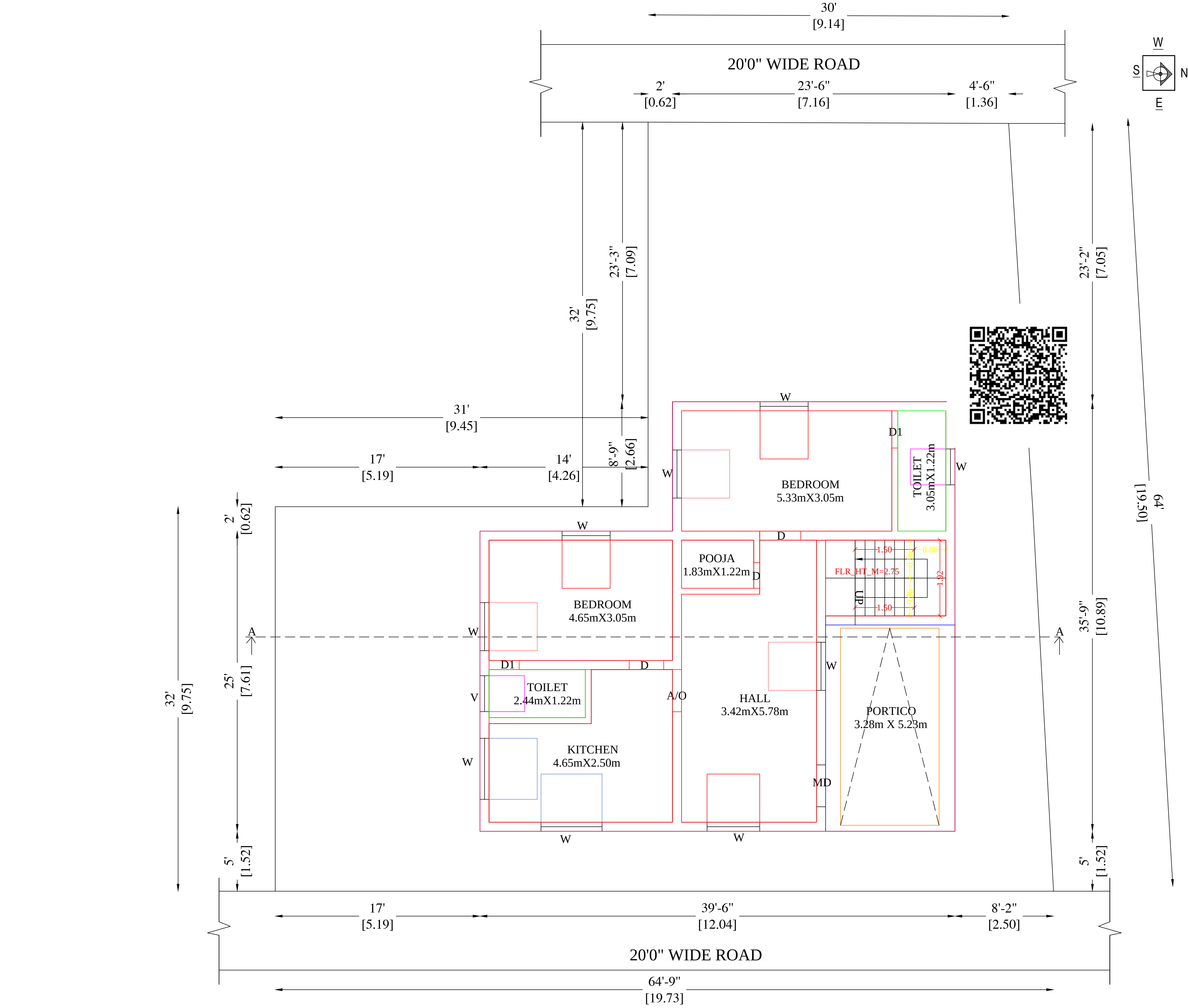
PRO. GROUND FLOOR PLAN
