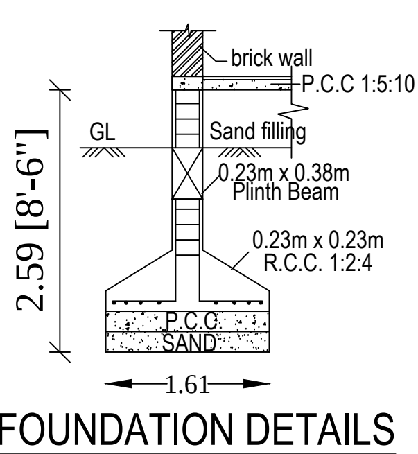
FOUNDATION DETAILS
