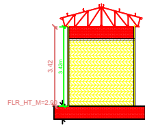
FRONT ELEVATION
