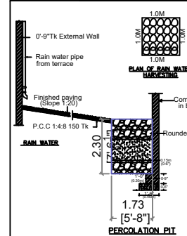
PERCOLATION PIT
