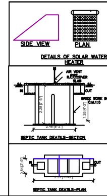
SEPTIC TANK DETAILS-PLAN
