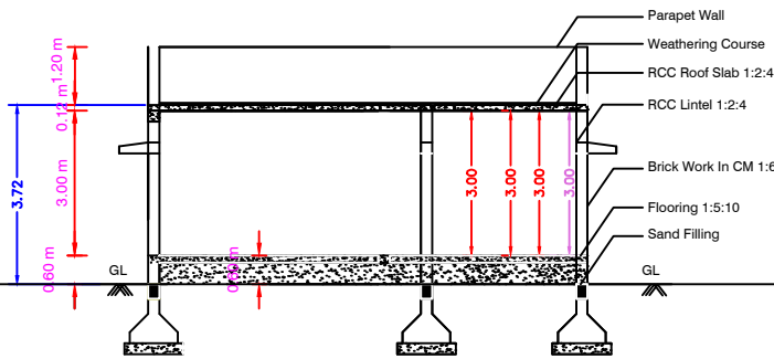
SECTION-AB
