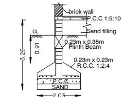
FOUNDATION DETAILS
