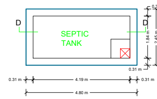
PLAN OF SEPTIC TANK SCALE 1"-20"
