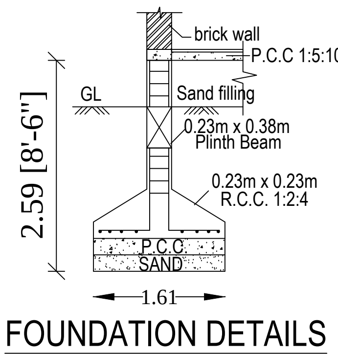
FOUNDATION DETAILS
