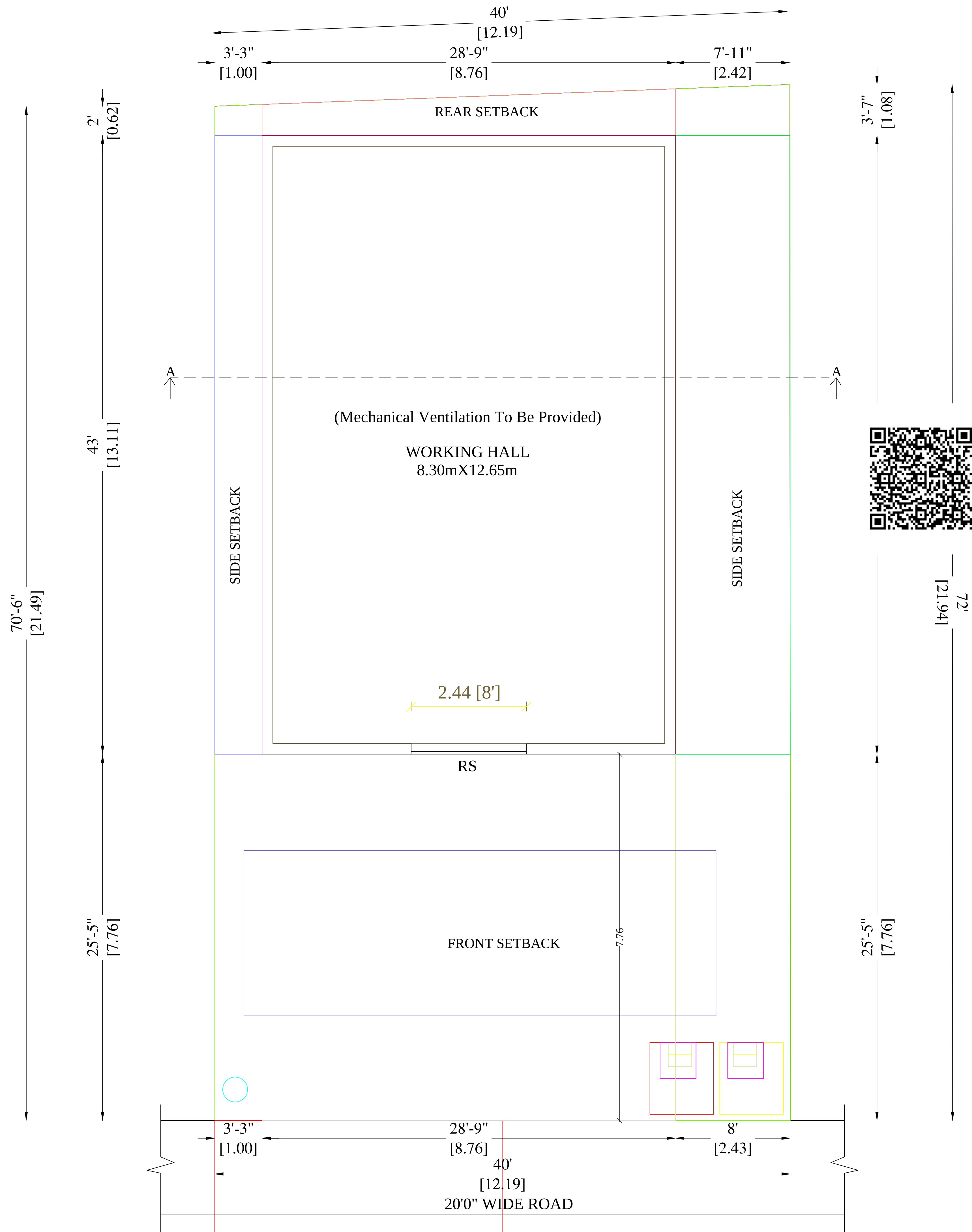
PRO. GROUND FLOOR PLAN
