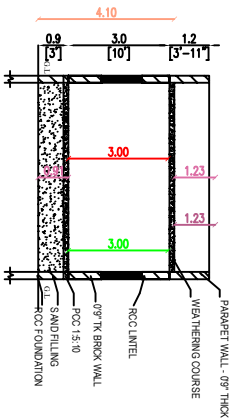
SECTION CUTTING XX
