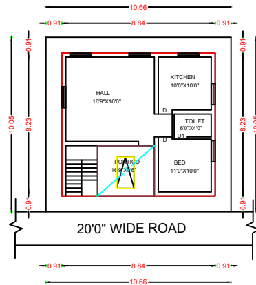
EXG .GROUND FLOOR PLAN
