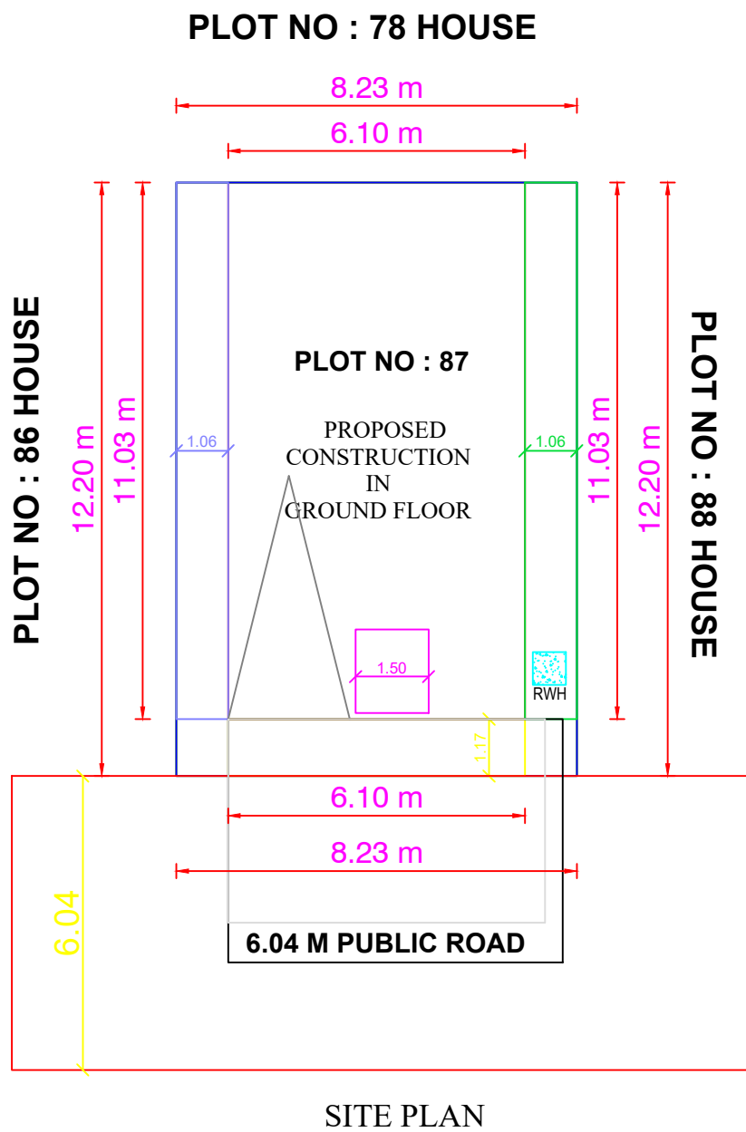
SITE PLAN
