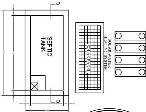
PLAN OF SEPTIC TANK SCALE 1"=2'-0"
