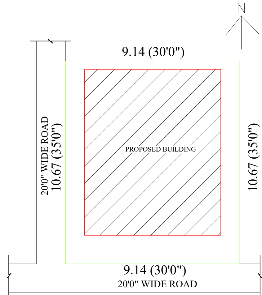
SITE PLAN
