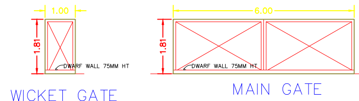
WICKET GATE
