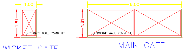
WICKET GATE
