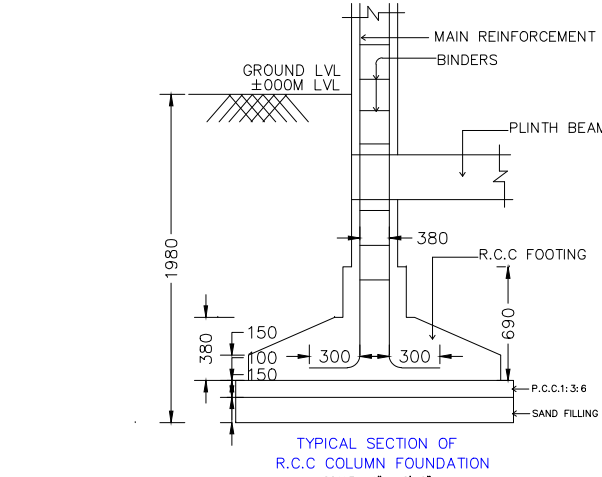
TYPICAL SECTION OF R.C.C. COLUMN FOUNDATION
