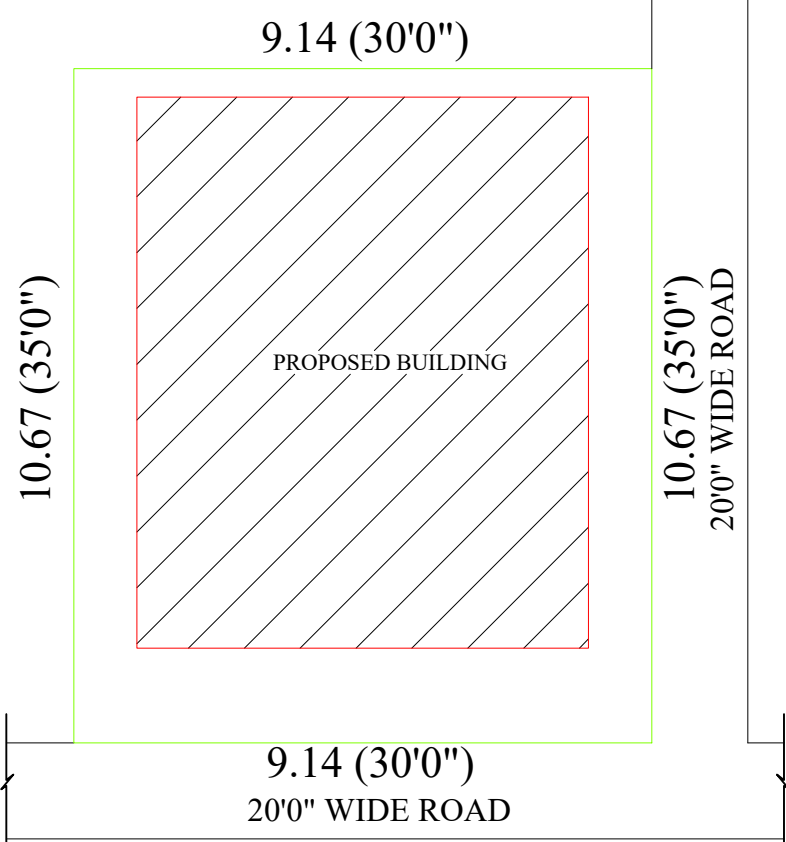
SITE PLAN
