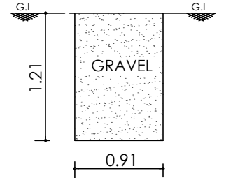
TRIAL PIT
