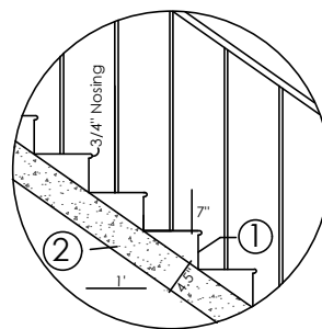
STAIRCASE SECTION
