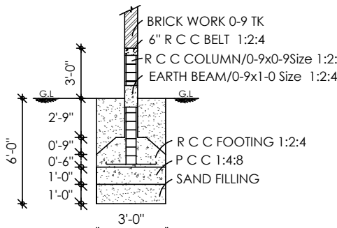
FOUNDATION
