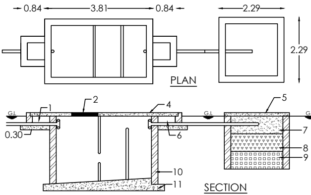
SEPTIC TANK
