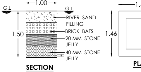
RAIN WATER HARVESTION
