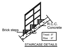
STAIRCASE DETAILS
