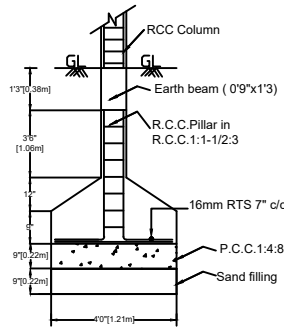
FOUNDATION DETAILS
