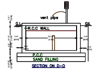
SECTION ON D-D
