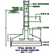
TYPICAL SECTION OF R.C.C. COLUMN FOUNDATION
