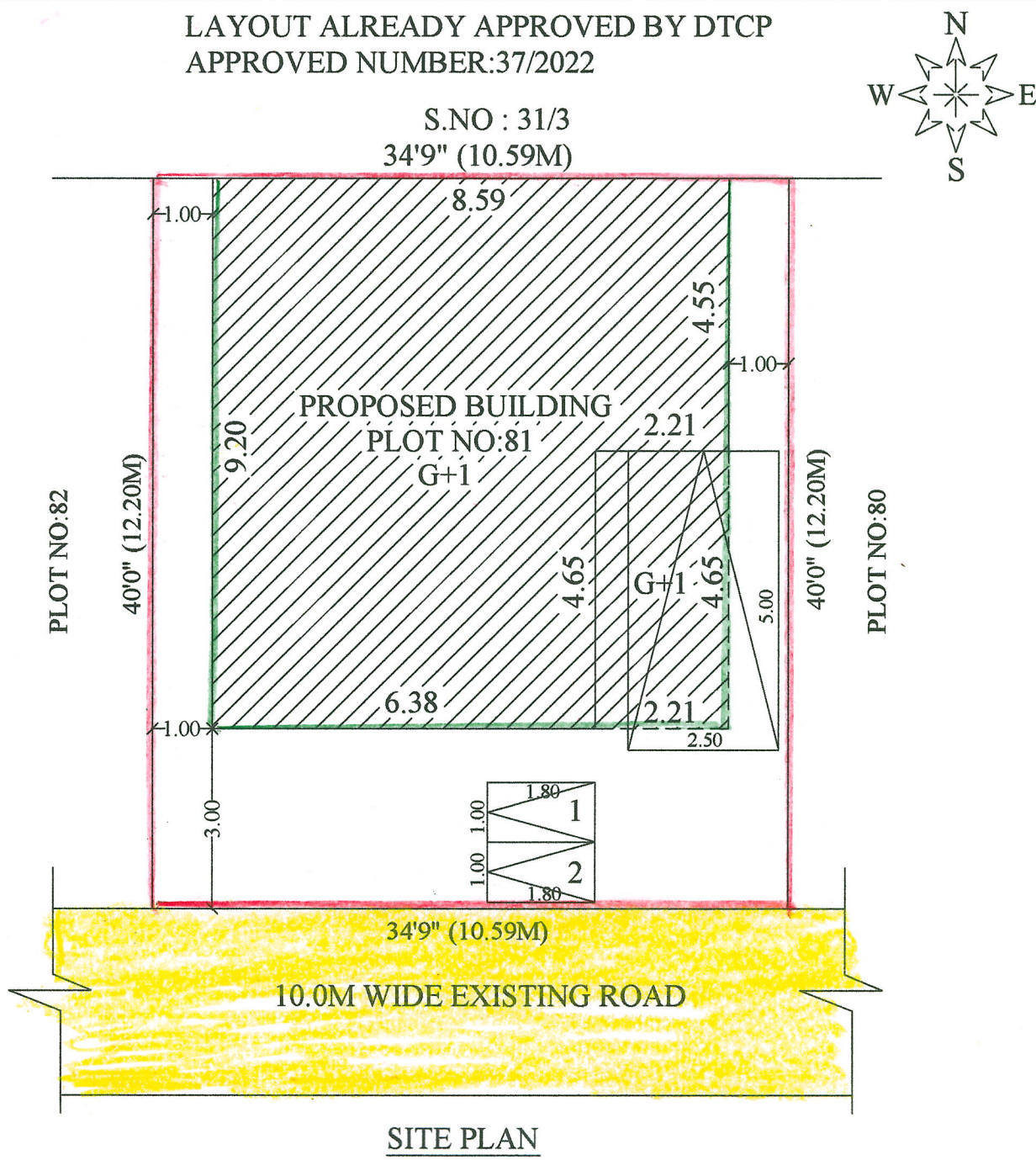
SITE PLAN
