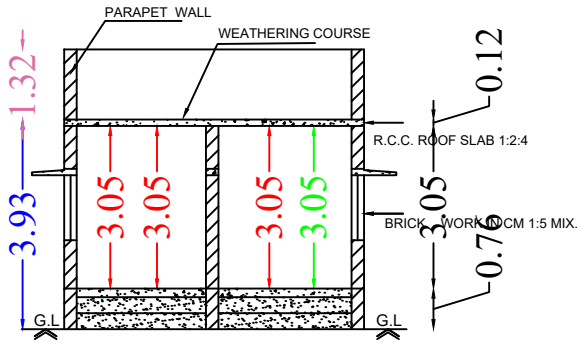
Section on-"AA"
