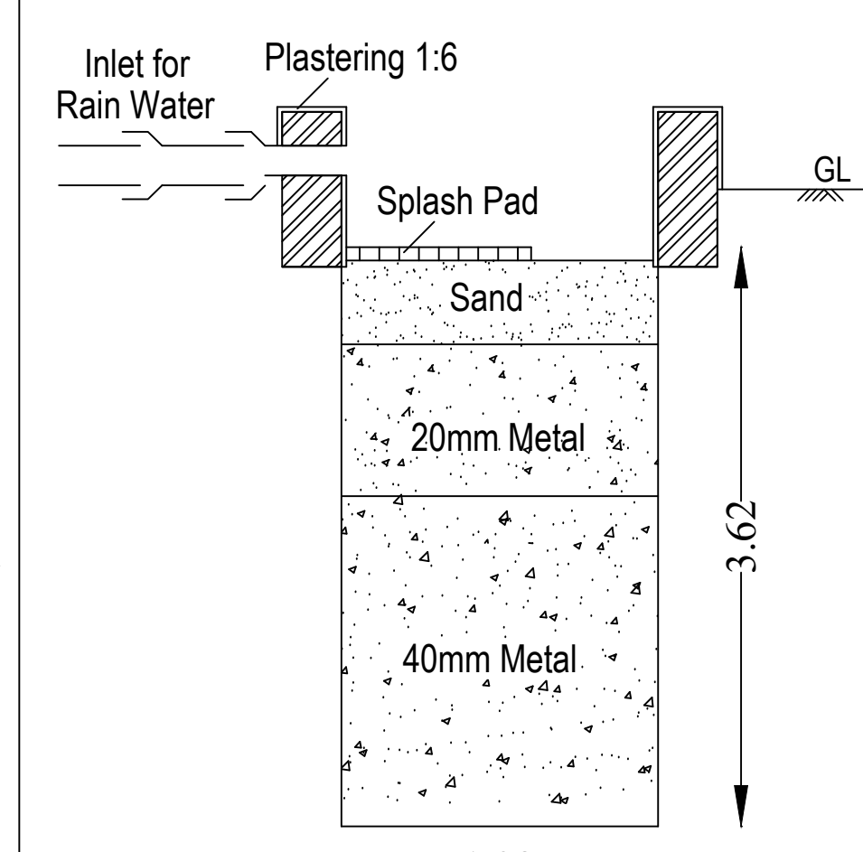
RAIN WATER PERCOLATION PIT
