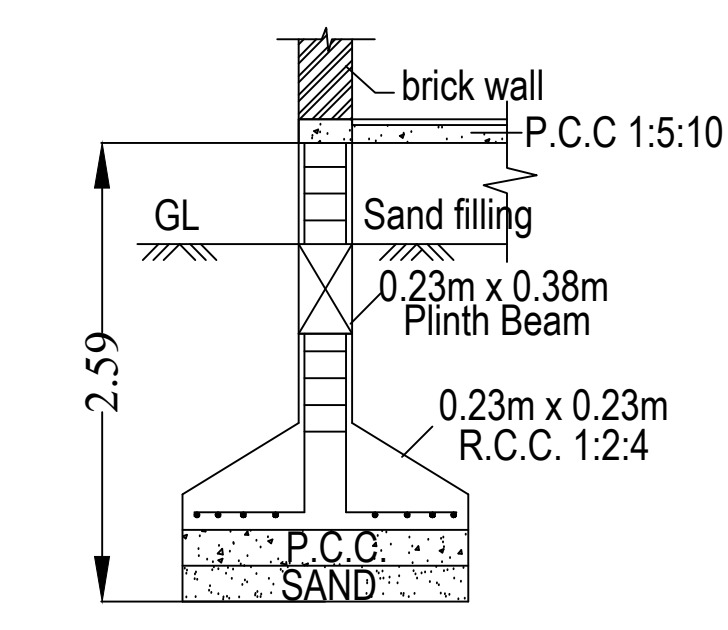
FOUNDATION DETAILS
