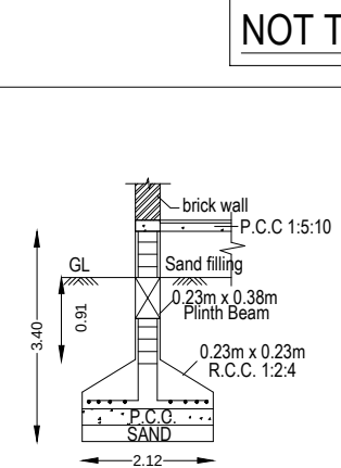
FOUNDATION DETAILS
