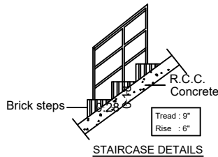
STAIRCASE DETAILS
