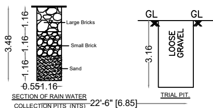
SECTION OF RAIN WATER COLLECTION PITS (NTS)
