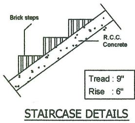
STAIRCASE DETAILS
