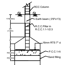
FOUNDATION DETAILS
