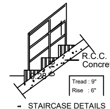
STAIRCASE DETAILS
