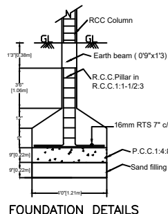
FOUNDATION DETAILS
