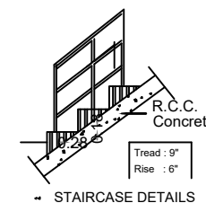
STAIRCASE DETAILS
