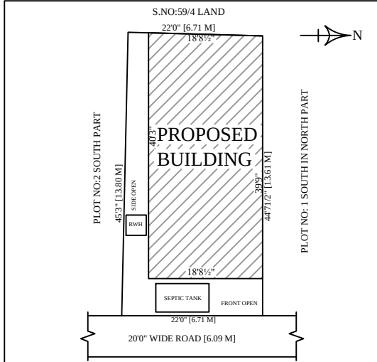
ENLARGED SITE PLAN
