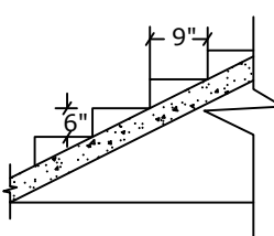
Staircase Detail Not To Scale
