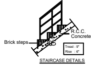
STAIRCASE DETAILS
