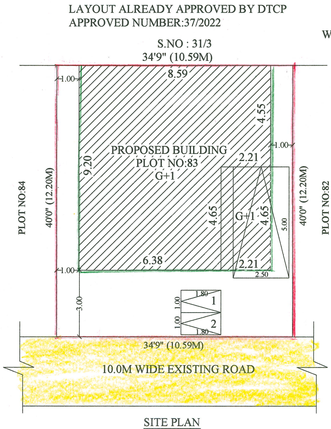
SITE PLAN
