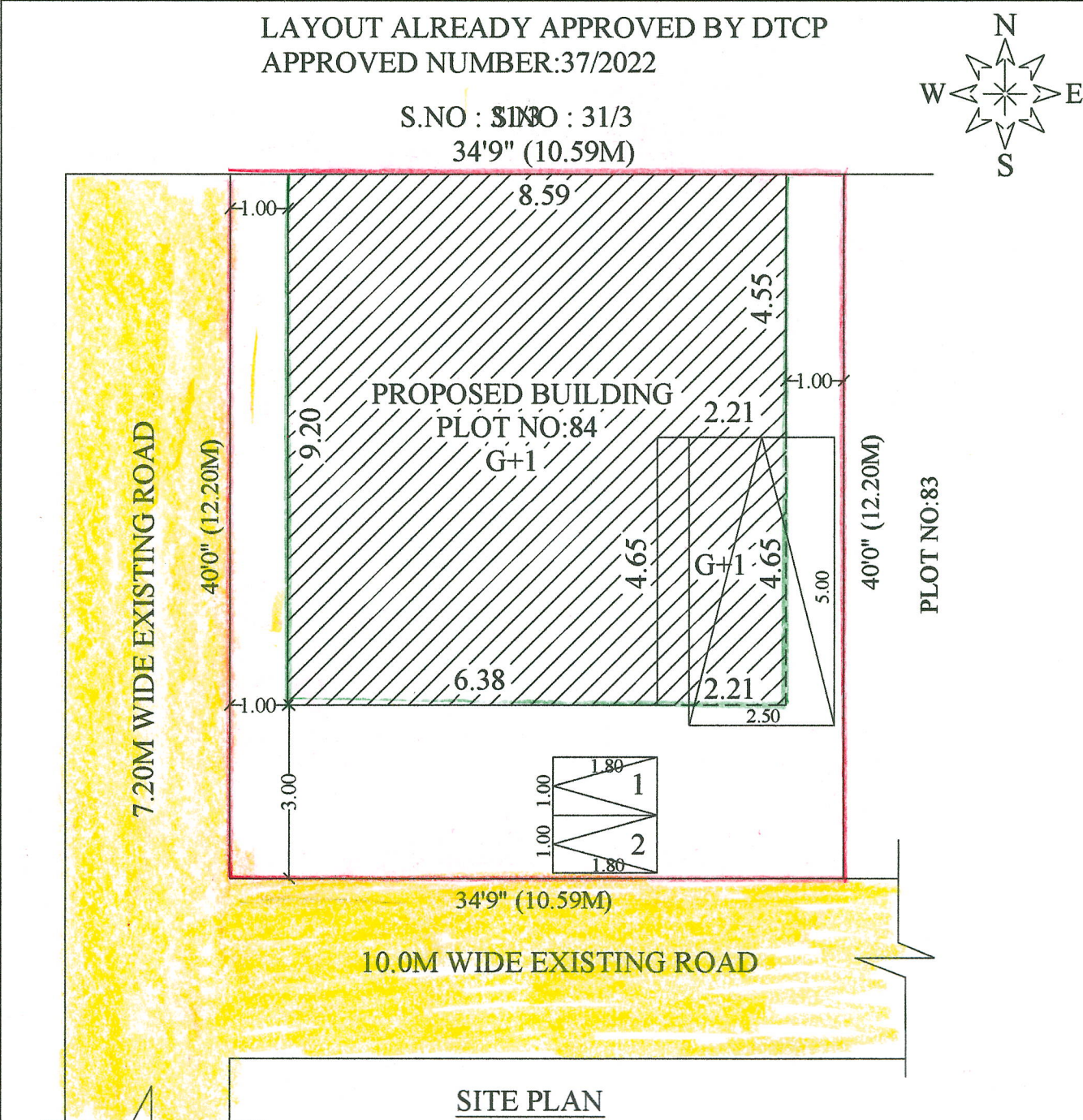
SITE PLAN
