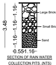
SECTION OF RAIN WATER COLLECTION PITS (INTS)
