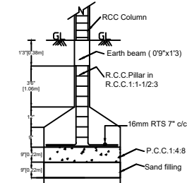
FOUNDATION DETAILS
