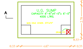
SUMP DETAIL SCALE 1"=4'-0"
