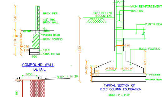
TYPICAL SECTION OF R.C.C. COLUMN FOUNDATION SCALE 1"=2'-0"
