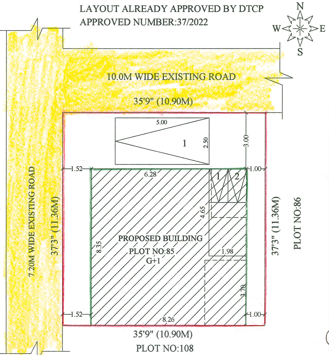
SITE PLAN
