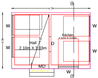
PROPOSED FIRST FLOOR
