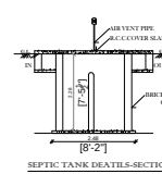
SEPTIC TANK DETAILS-SECTION
