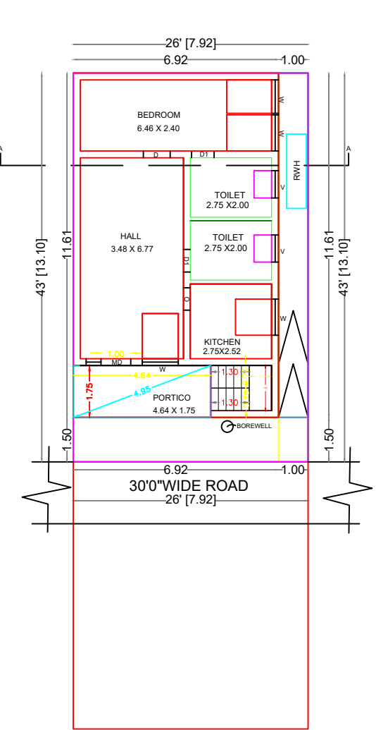
PRO. GROUND FLOOR PLAN
