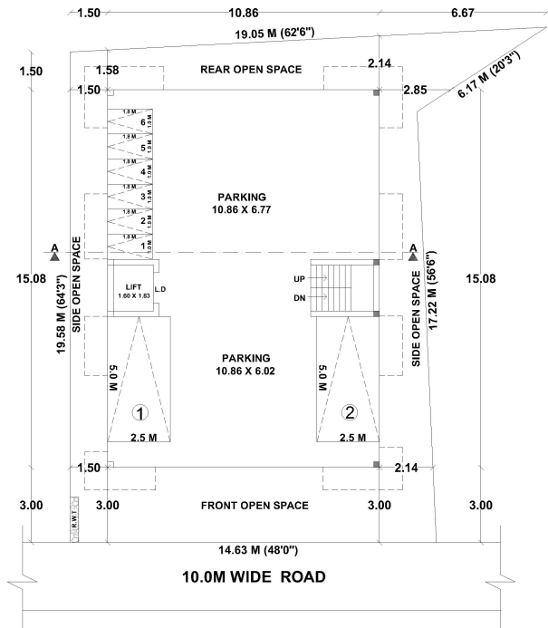
STILT FLOOR PLAN
