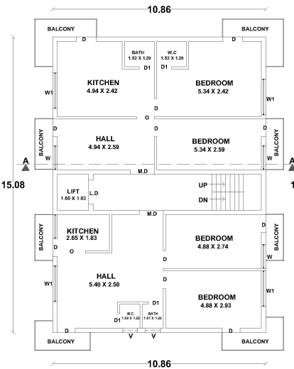
TYPICAL FLOOR PLAN (FIRST, SECOND & THIRD)
