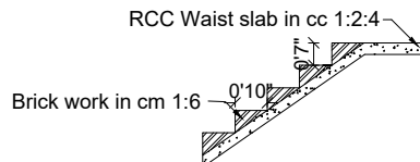
STAIRCASE DETAILS (Not to Scale)
