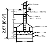
FOUNDATION DETAILS
