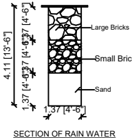
SECTION OF RAIN WATER
