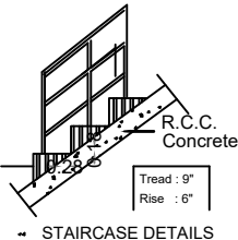
STAIRCASE DETAILS
