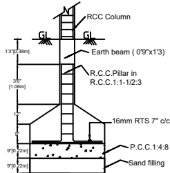
FOUNDATION DETAILS
