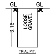
TRIAL PIT
