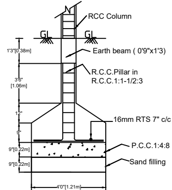
FOUNDATION DETAILS
