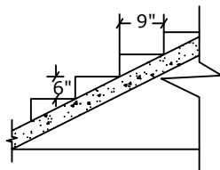
Staircase Detail Not To Scale
