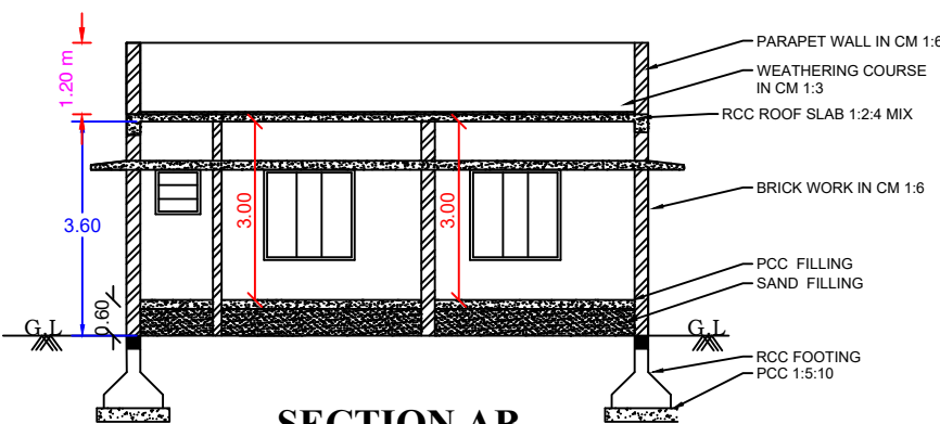
SECTION AB
