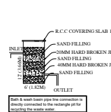
SECTION - 'CD'
