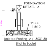
FOUNDATION DETAIL - A
