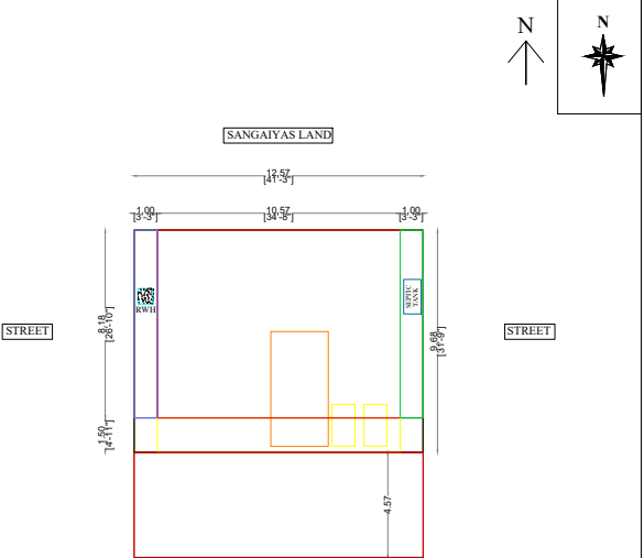
Site Plan
